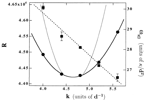
FIG. 4. Marginal stability boundary in parameter space of R and azimuthal wave number k (●) and \omega_{\kappa 0} vs k (■) for \Omega = 544 with \Gamma = 2.5 . The solid line is a nonlinear third-order polynomial fit to the marginal stability data, the short-dashed line is the finite-size Eckhaus boundary, and the long-dashed line is a linear fit to the frequencies.
