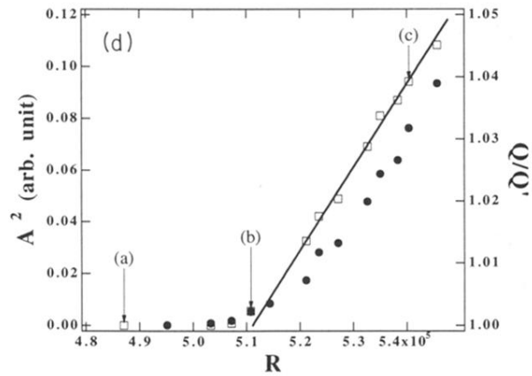
FIG. 7. Shadowgraph images of convection pattern (a) below ( R = 4.87 \times 10^5 , \epsilon = -0.062 ), (b) nearly at ( R = 5.11 \times 10^5 , \epsilon = -0.016 ), and (c) above ( R = 5.38 \times 10^5 , \epsilon = 0.037 ) the onset of bulk convection, and (d) the effective Nusselt number Q/Q' ( \bullet ), i.e., the ratio of the total heat conducted in the convecting state divided by the heat conducted by the sidewall state alone, and the squared amplitude ( \square ) vs \epsilon . All the data are for \Omega = 2145 and the \epsilon values for the patterns are labeled in (d).
