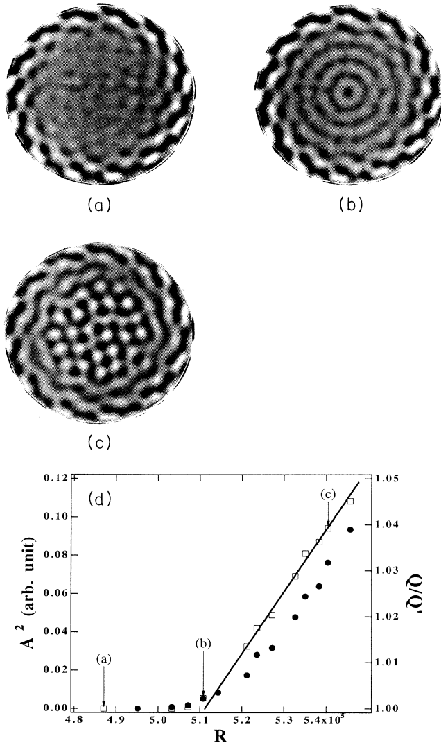
FIG. 7. Shadowgraph images of convection pattern (a) below ( R = 4.87 \times 10^5 , \epsilon = -0.062 ), (b) nearly at ( R = 5.11 \times 10^5 , \epsilon = -0.016 ), and (c) above ( R = 5.38 \times 10^5 , \epsilon = 0.037 ) the onset of bulk convection, and (d) the effective Nusselt number Q/Q' ( \bullet ), i.e., the ratio of the total heat conducted by the convecting state divided by the heat conducted by the sidewall state alone, and the squared amplitude ( \square ) vs \epsilon . All the data are for \Omega = 2145 and the \epsilon values for the patterns are labeled in (d).
