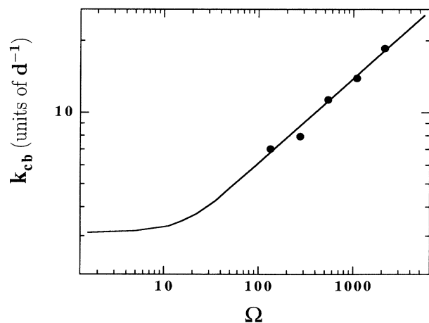
FIG. 6. The critical bulk wave number k_{cb} vs \Omega for the bulk state obtained from shadowgraph images. The solid line is from Chandrasekhar (Ref. [1]).
