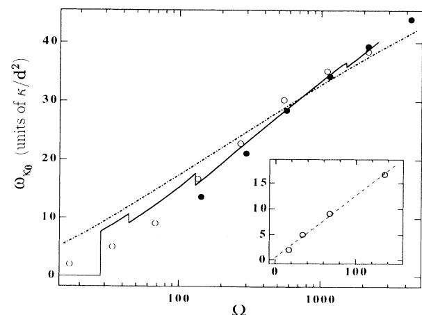
FIG. 2. Comparison of experimental and theoretical results on the precession frequencies of the wall convection states. Data for a cell with an aspect ratio of 2.5 ( \circ ) and 1 ( \bullet ), the results of Goldstein et al. ( — ) for a unit-aspect-ratio cell, and the results of Kuo and Cross ( - - - ) for a planar wall state. The inset is a linear plot of the frequencies at small rotation rate and the dashed line is a fit to the data.
