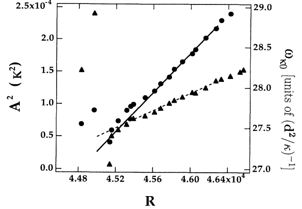
FIG. 5. Temperature amplitude squared A^2 (●) and frequency \omega_{\kappa 0} (▲) vs R for the transition from mode 13 to mode 12.
