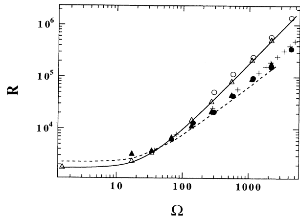
FIG. 1. Parameter-space diagram of rotating Rayleigh-Bénard convection in small-aspect-ratio cylindrical containers. Measured bifurcation points from conduction to wall convection ( \blacktriangle ) and bulk convection states ( \triangle ) for a cell with an aspect ratio of 2.5 and corresponding bifurcation points ( \bullet and \circ ) measured in a unit-aspect-ratio cell (Ref. [4]) are shown. Rossby's results ( + ) for aspect ratios 1.4–5 (Ref. [3]), Chandrasekhar's linear stability calculation for a laterally infinite system ( — ), and the result of Goldstein et al. ( - - - ) for a unit-aspect-ratio cell with insulating sidewalls (Ref. [10]) are also shown for comparison.
