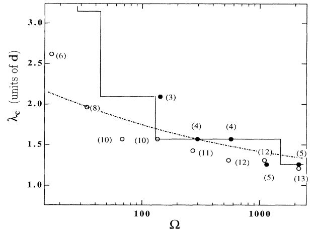
FIG. 3. The critical wavelength for wall convection states with \Gamma=2.5 (o) and \Gamma=1 (•). The bracketed numbers are the corresponding mode numbers. The solid line is from Goldstein et al. for a unit-aspect-ratio cell and the dash-dotted curve is from Kuo and Cross for a planar wall state.
